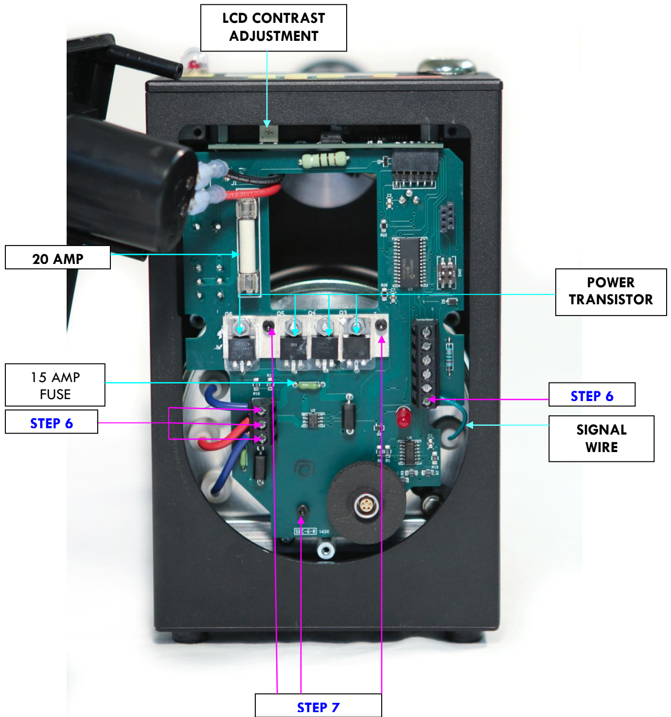
Oscillator Board
