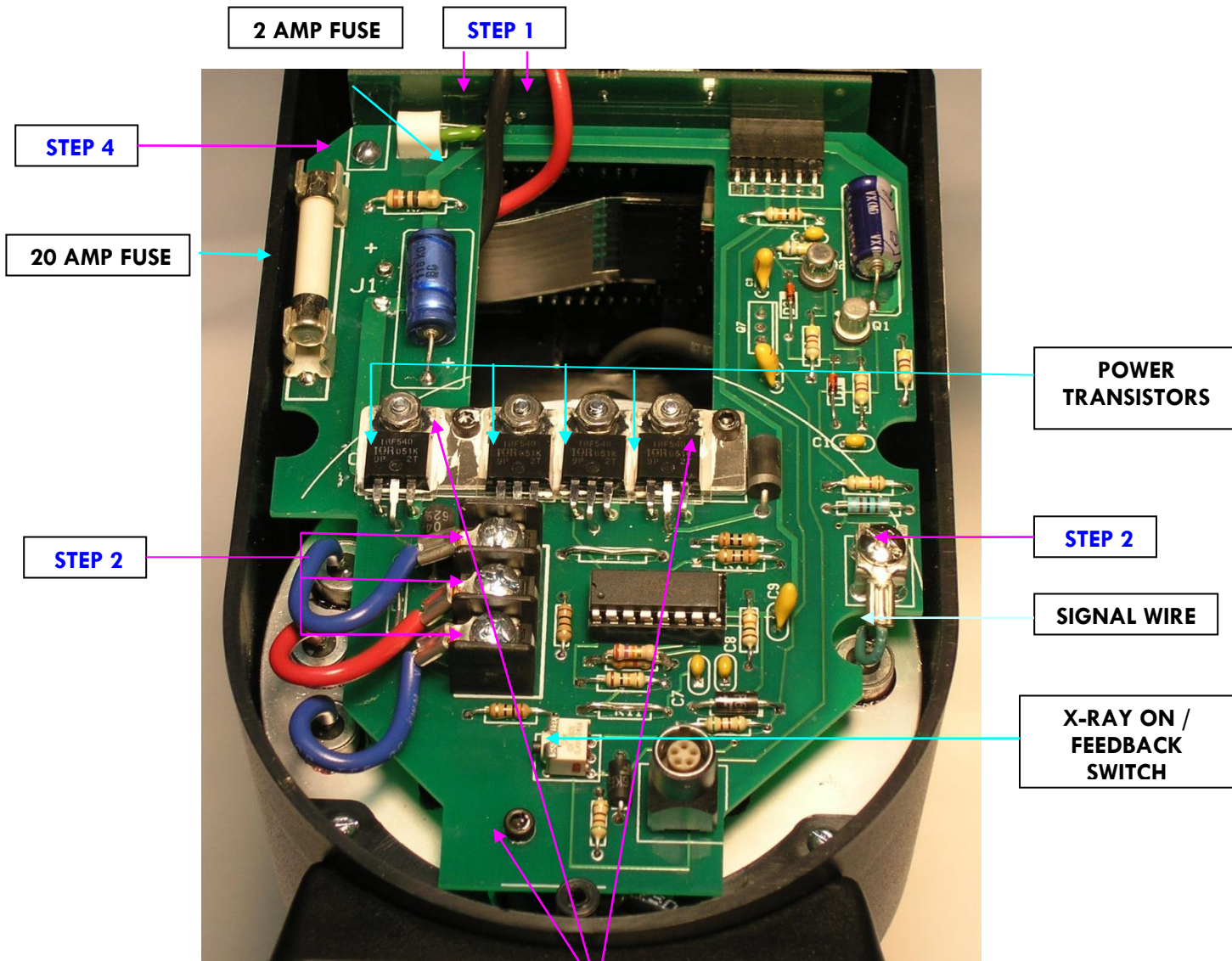
Figure 7: Oscillator Board
